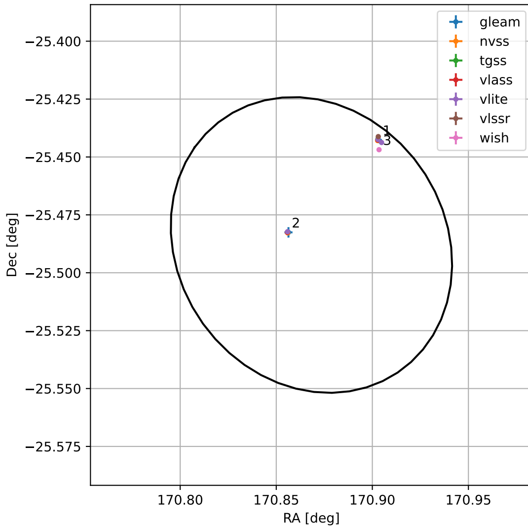
4FGL J1123.4-2529
