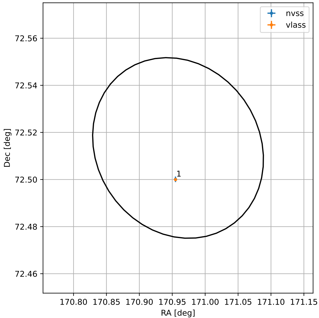
4FGL J1123.8+7230
