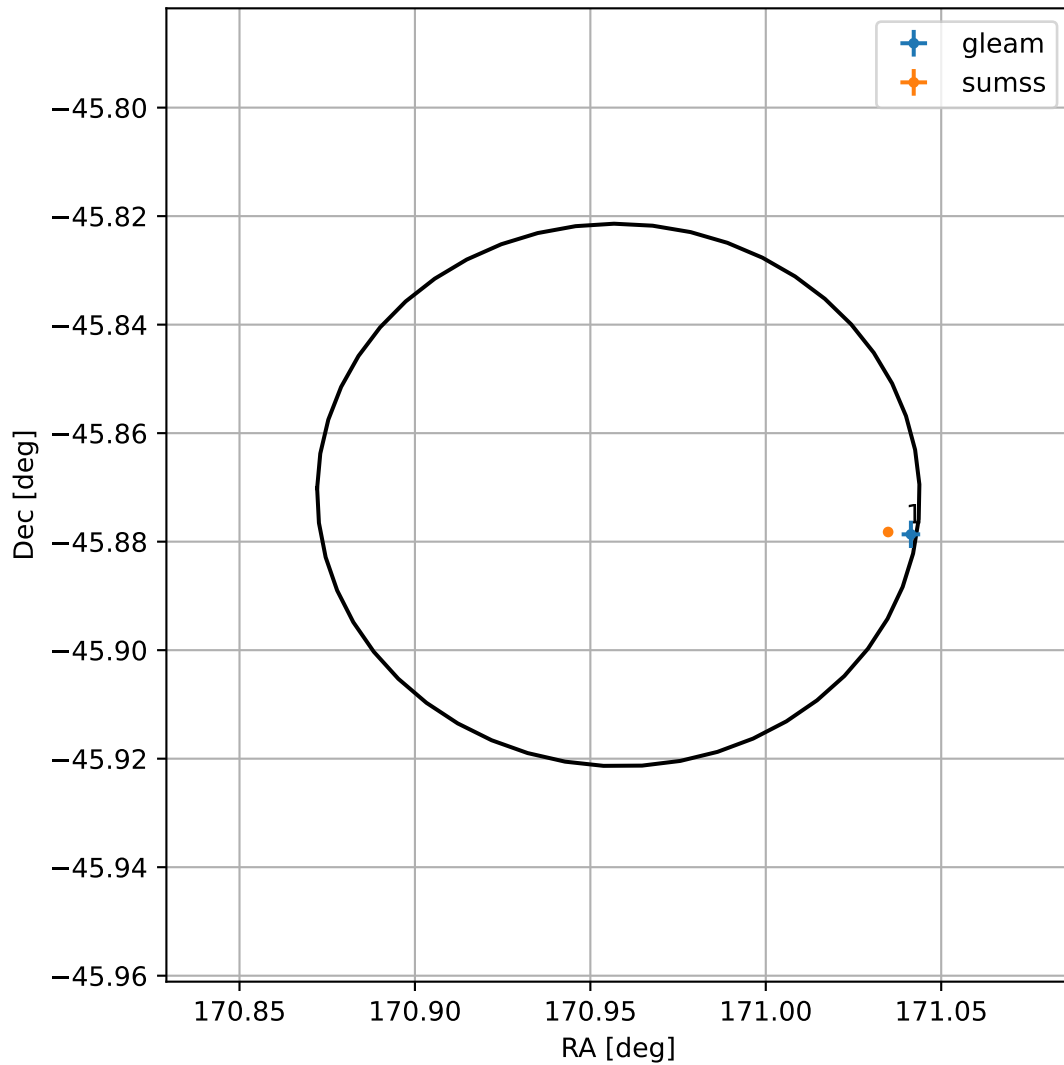
4FGL J1123.8-4552
