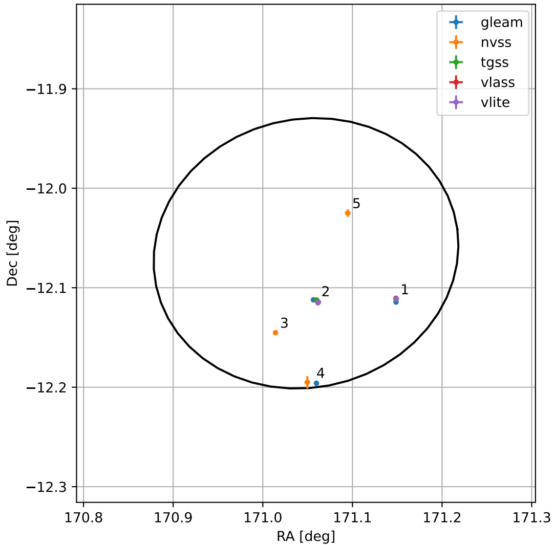
4FGL J1124.1-1203
