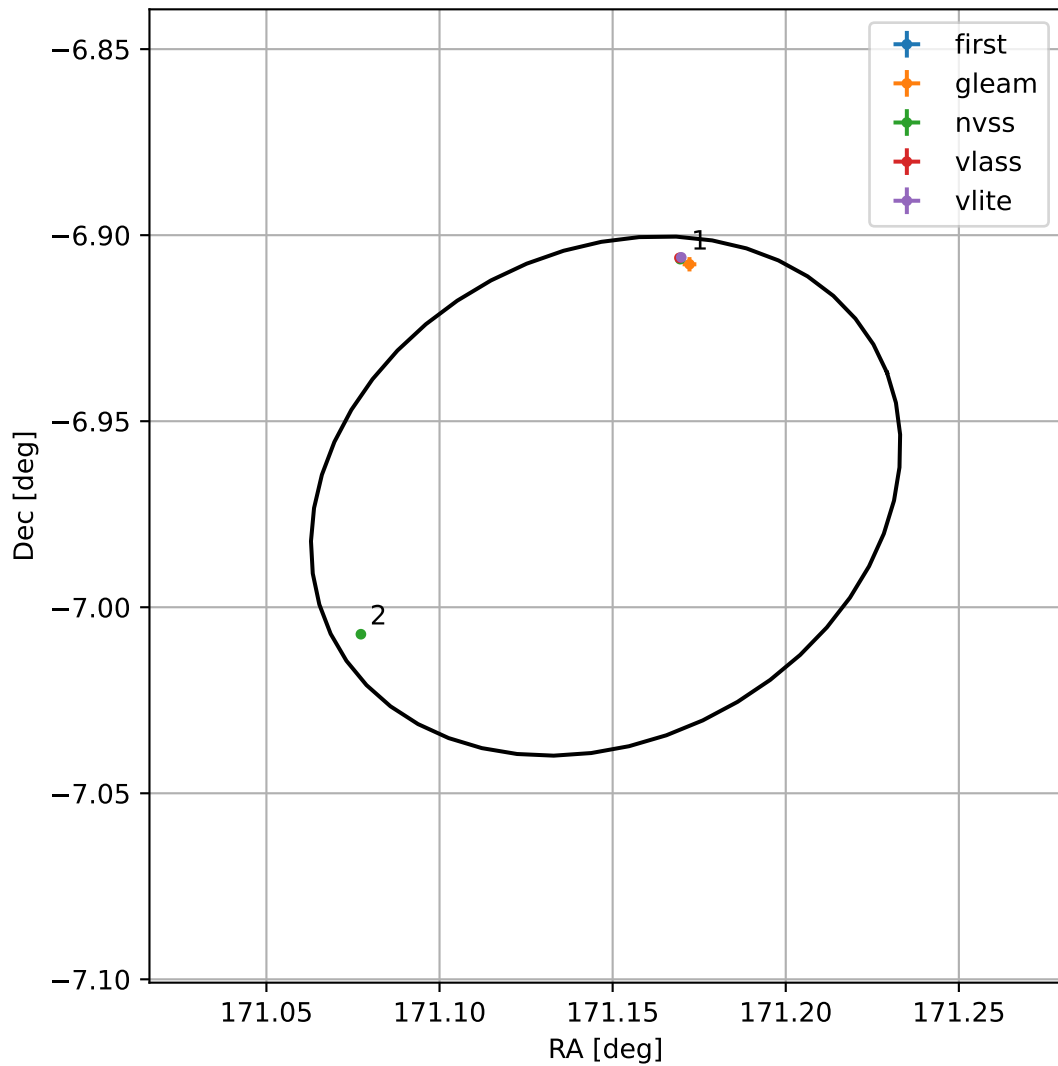
4FGL J1124.5-0658
