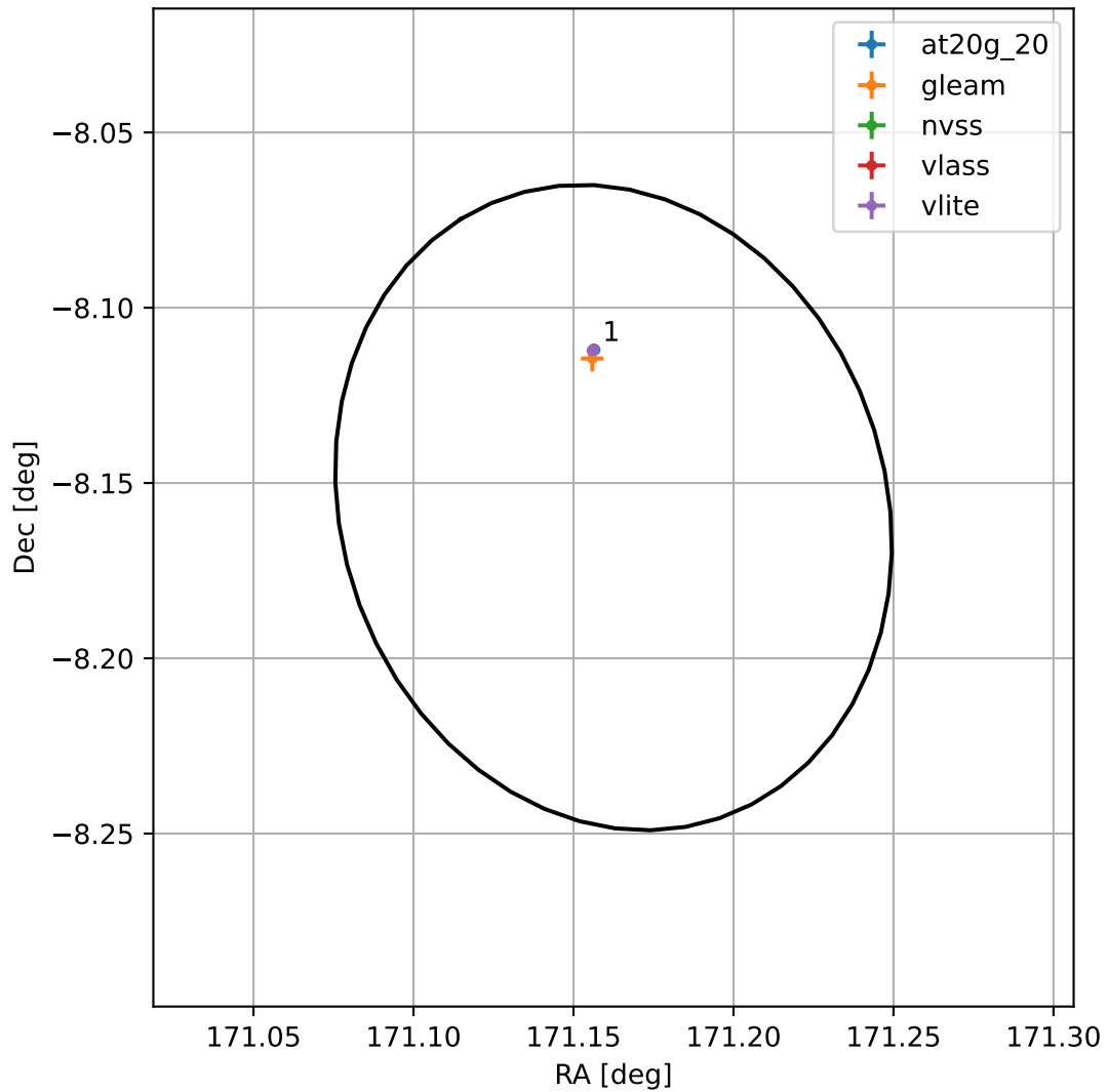
4FGL J1124.6-0809
