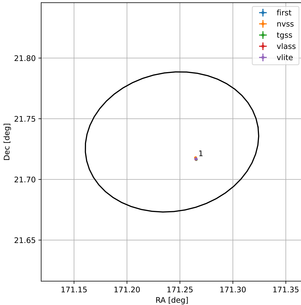
4FGL J1124.9+2143
