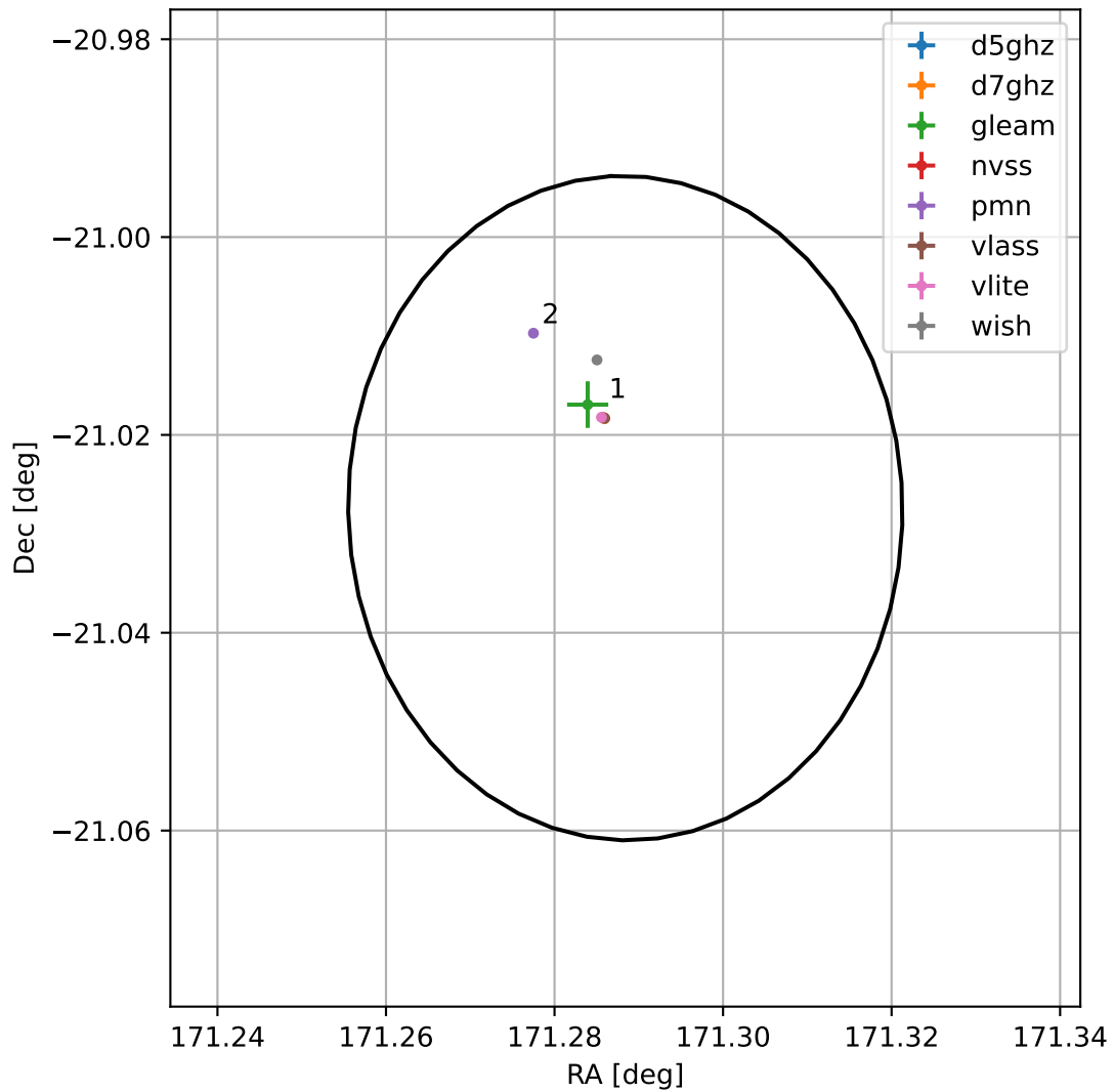
4FGL J1125.1-2101
