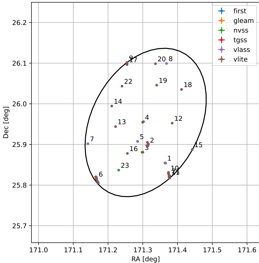
4FGL J1125.2+2557
