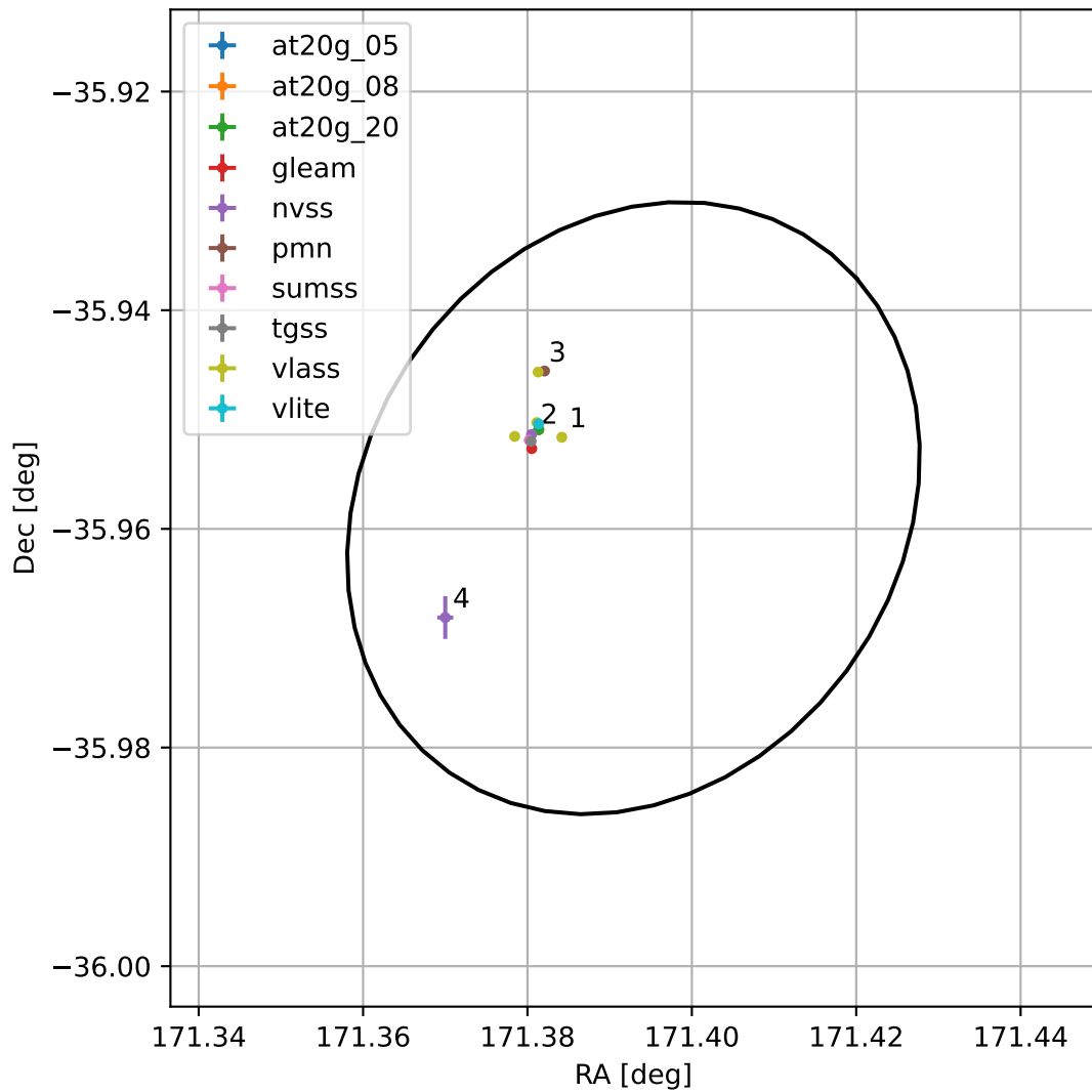
4FGL J1125.5-3557
