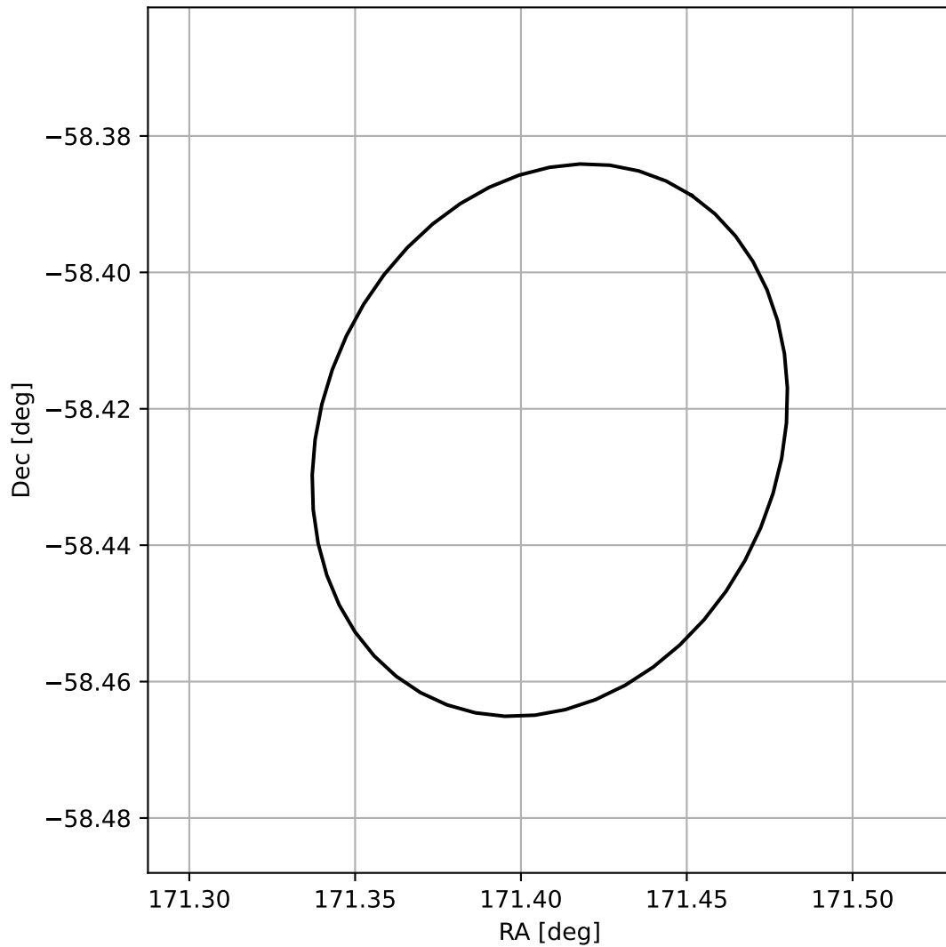
4FGL J1125.6-5825
