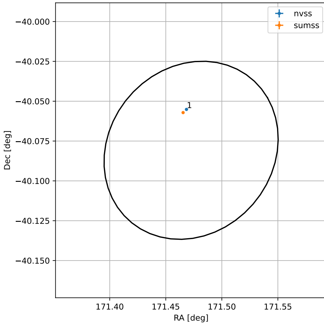
4FGL J1125.8-4004
