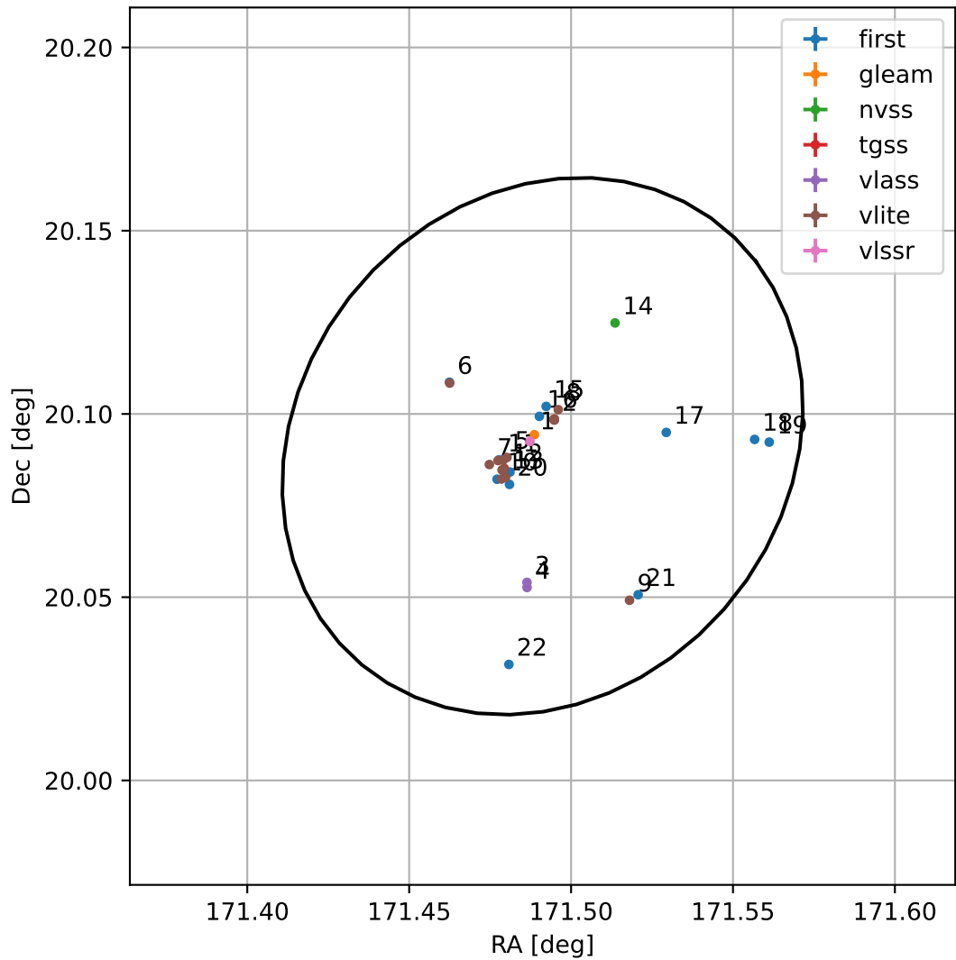
4FGL J1125.9+2005
