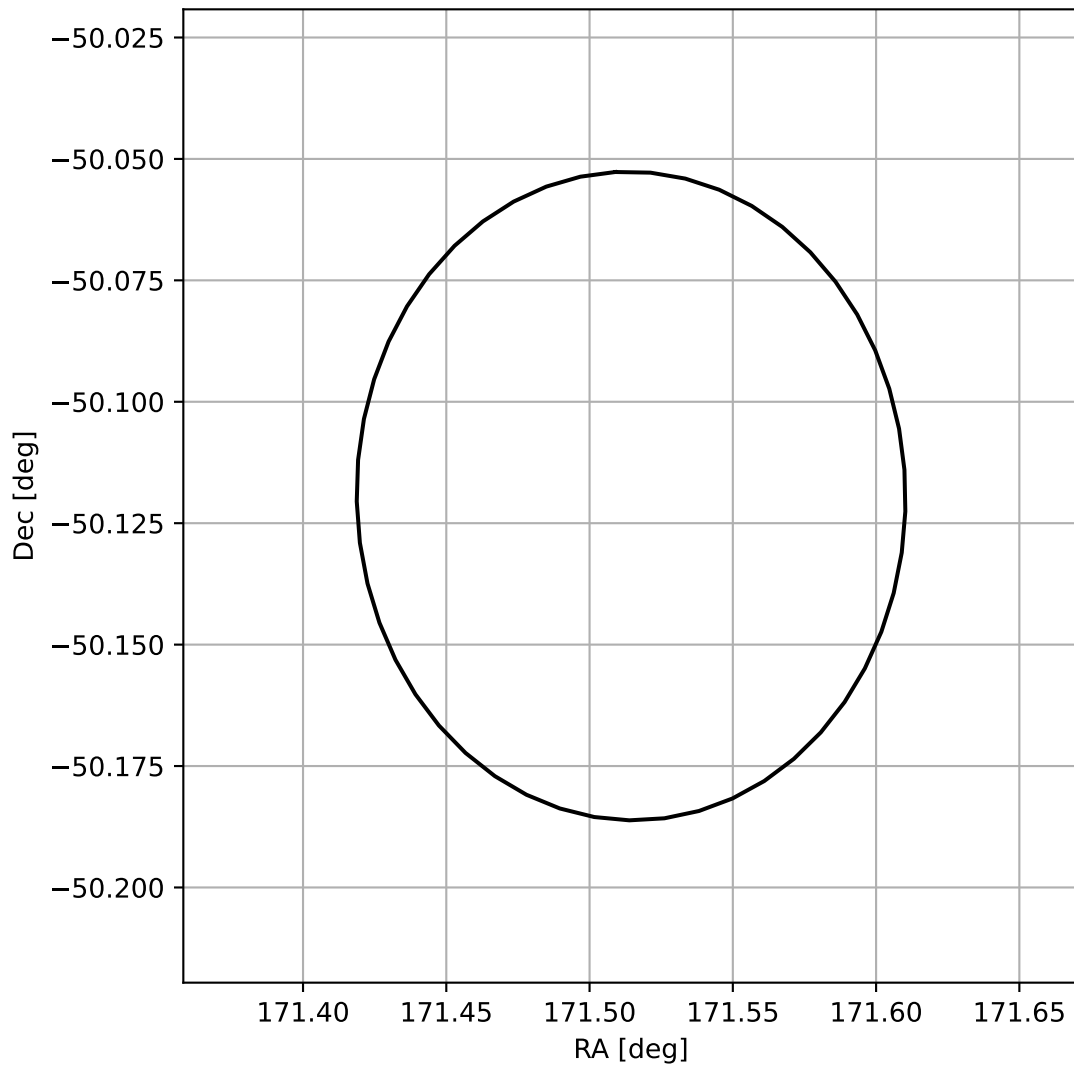
4FGL J1126.0-5007
