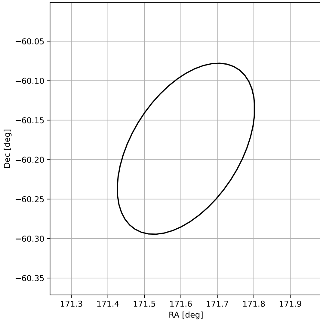
4FGL J1126.4-6011
