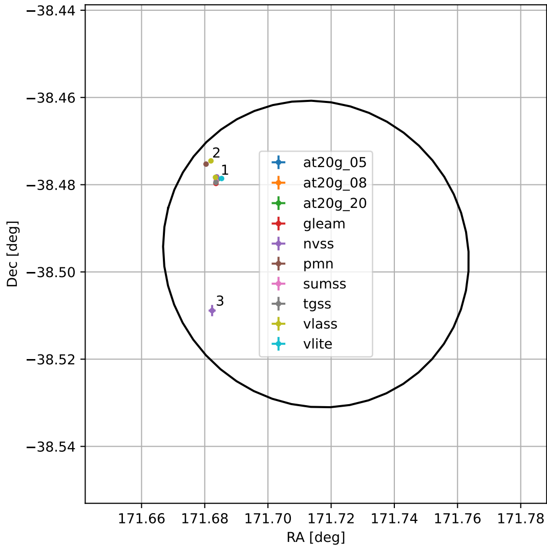
4FGL J1126.8-3829
