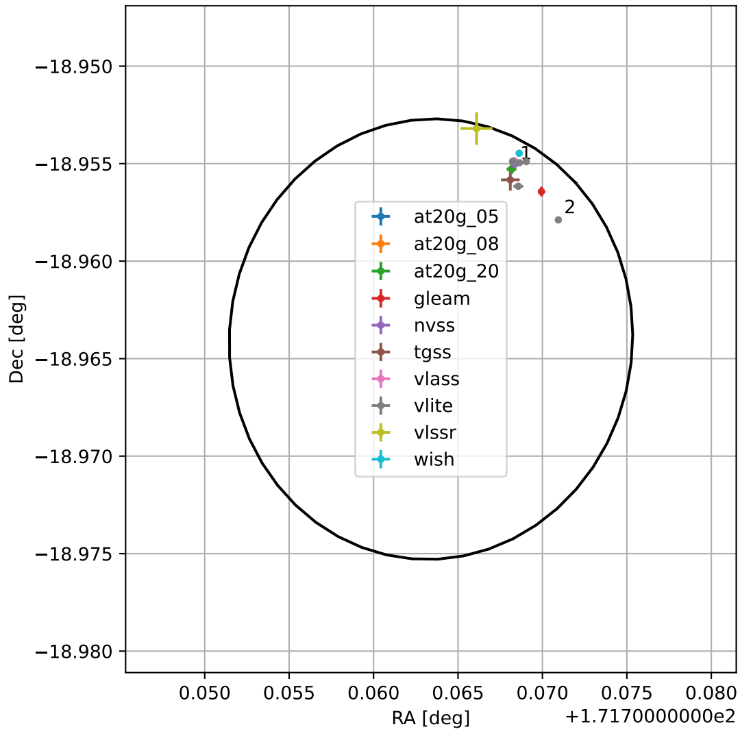
4FGL J1127.0-1857
