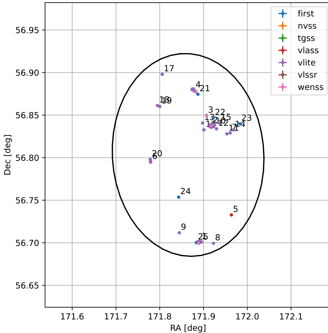
4FGL J1127.4+5648
