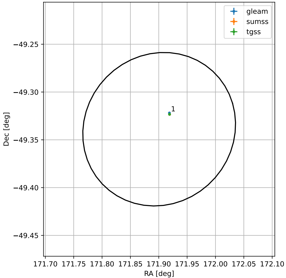
4FGL J1127.6-4920
