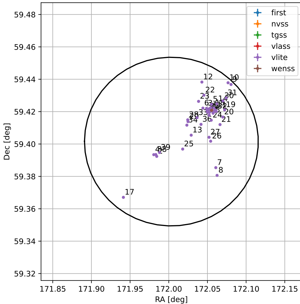
4FGL J1128.0+5924
