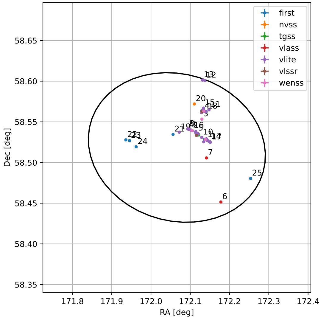
4FGL J1128.2+5831
