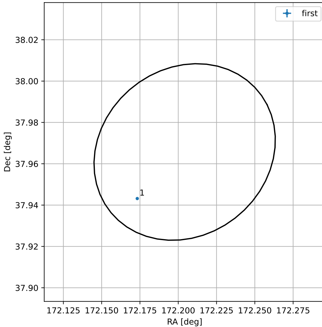
4FGL J1128.8+3757
