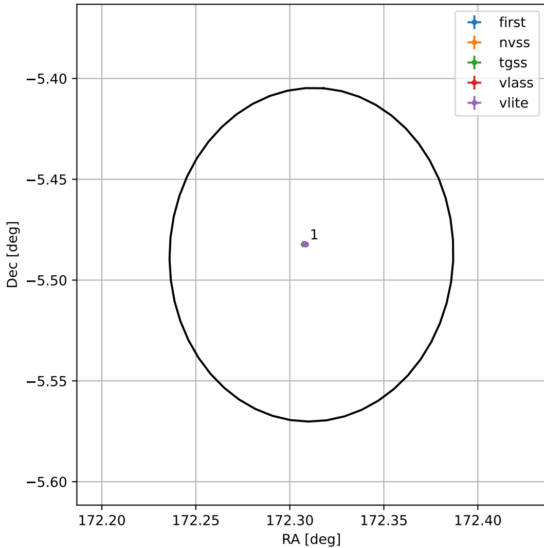
4FGL J1129.2-0529
