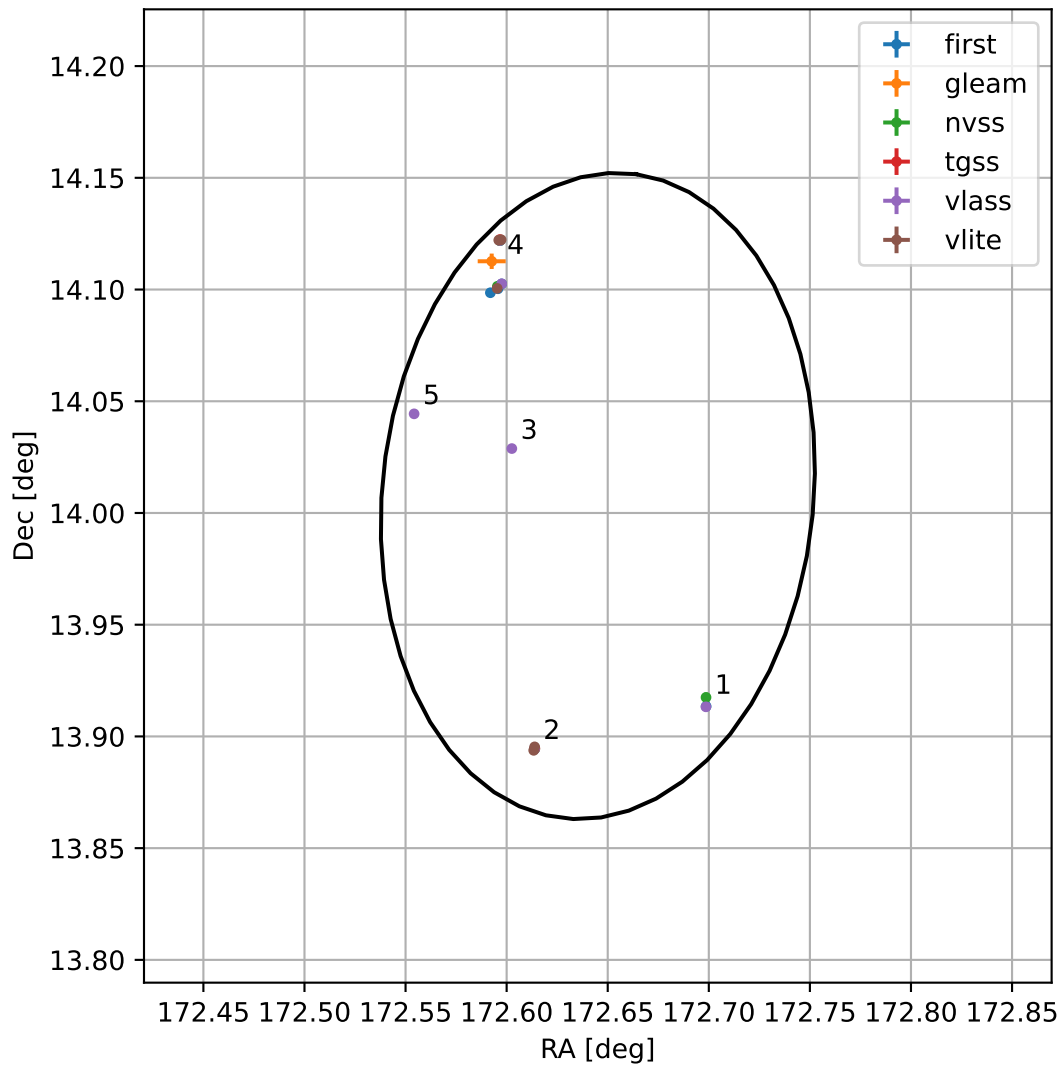
4FGL J1130.5+1400
