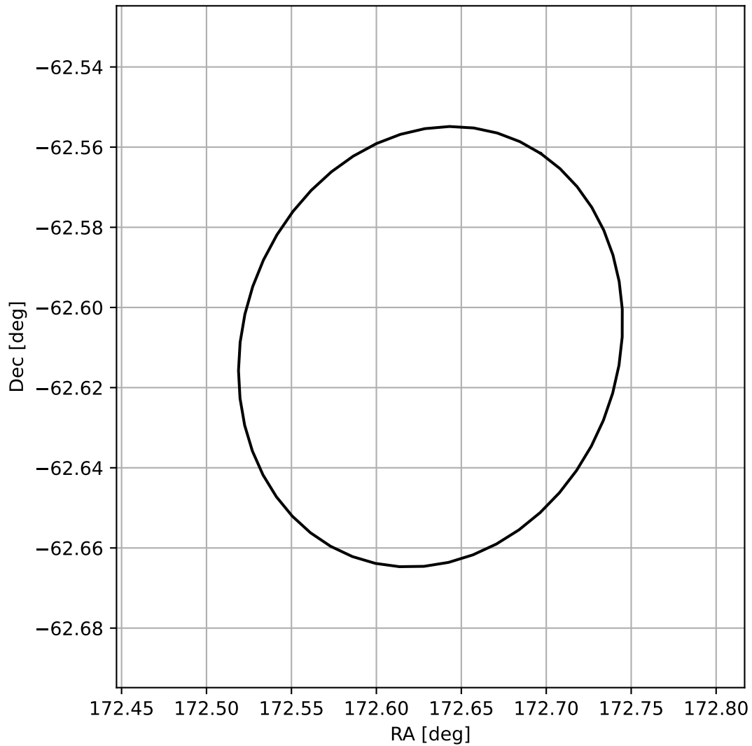
4FGL J1130.5-6236
