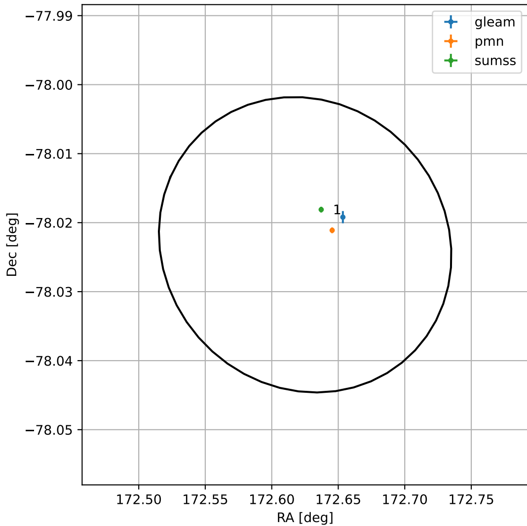
4FGL J1130.5-7801
