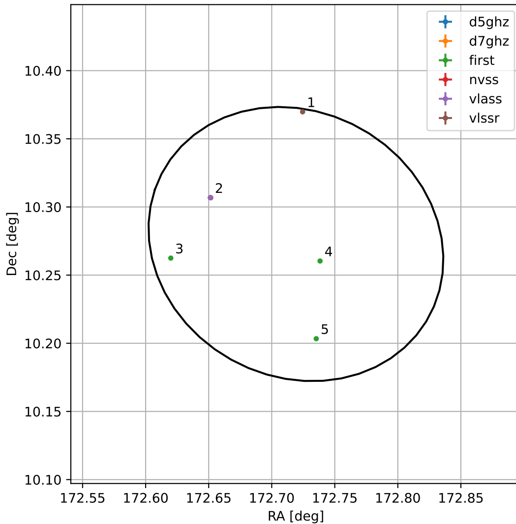
4FGL J1130.8+1016
