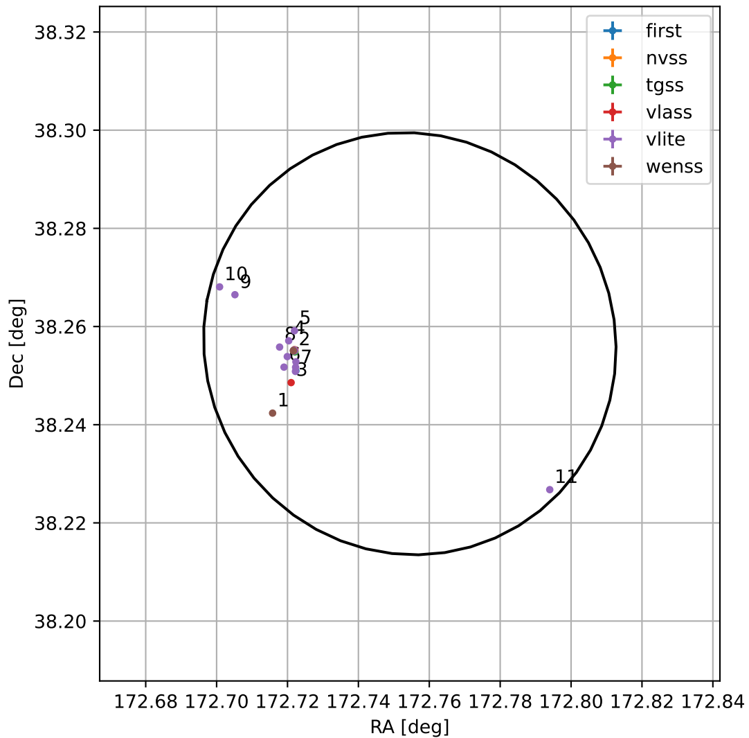
4FGL J1131.0+3815
