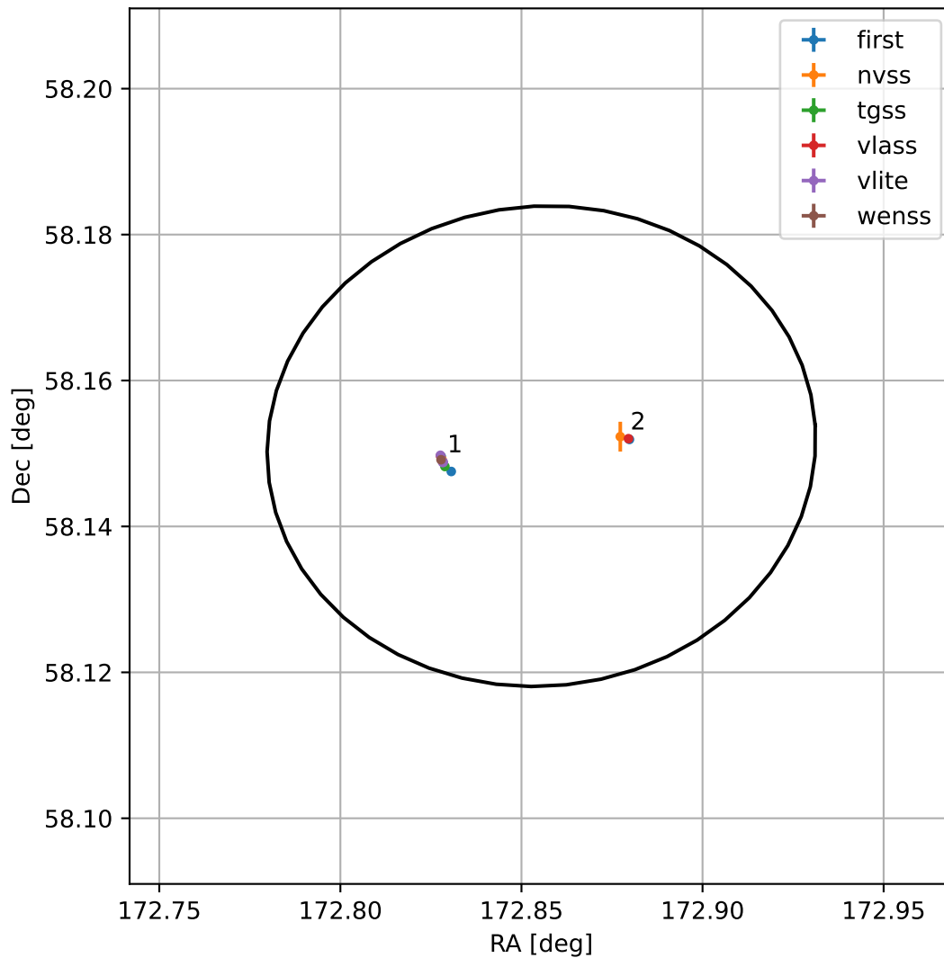
4FGL J1131.4+5809
