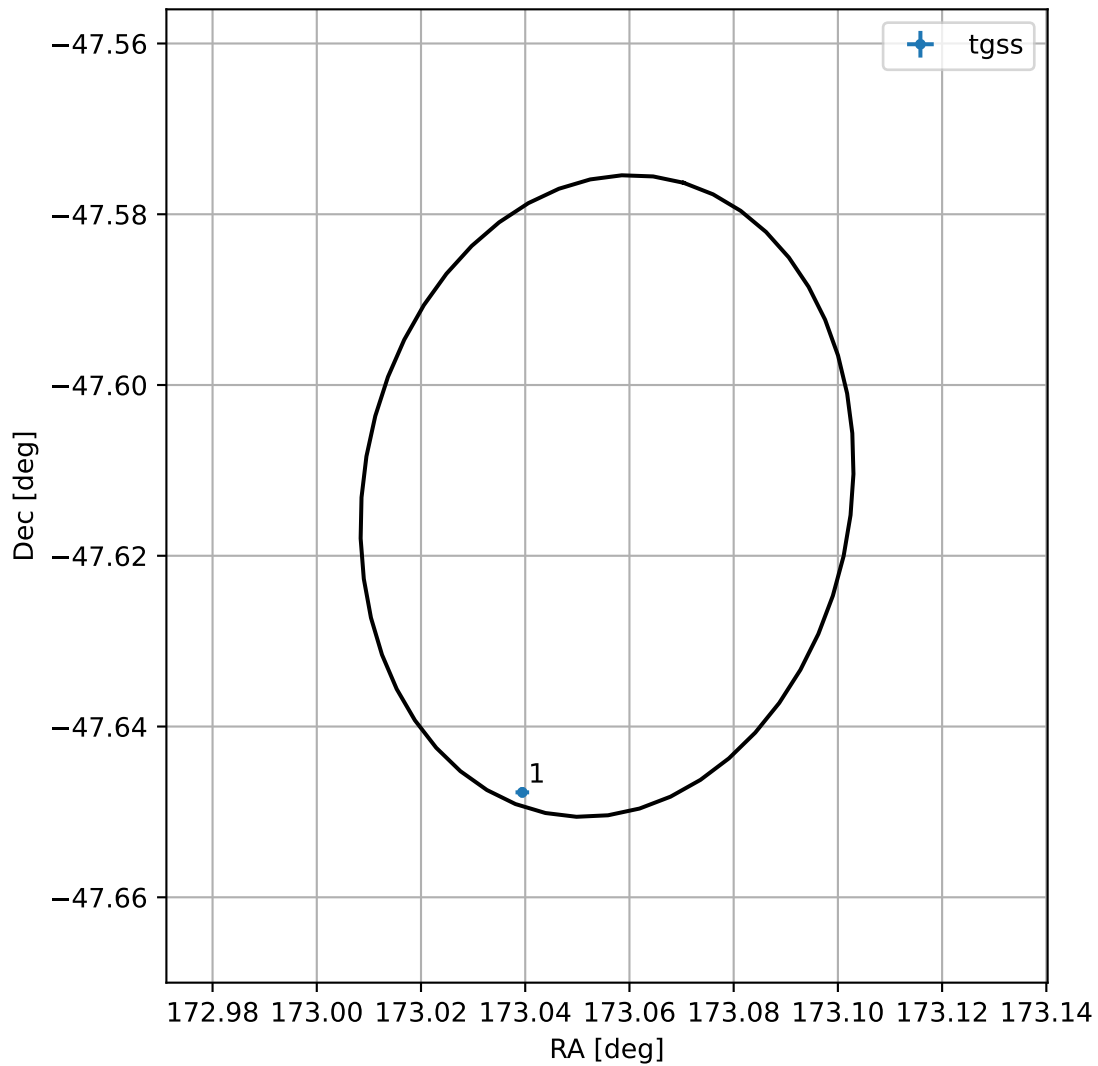
4FGL J1132.2-4736
