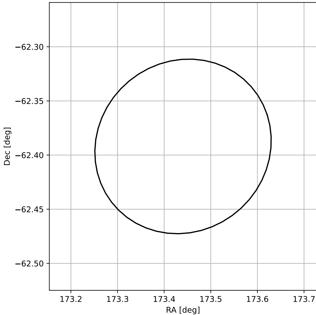
4FGL J1133.7-6223
