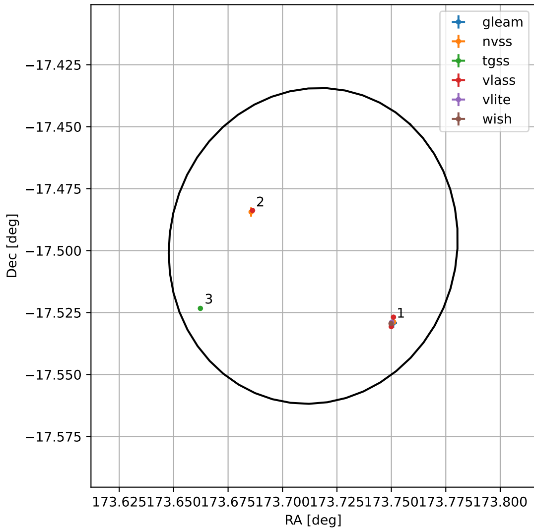
4FGL J1134.8-1729
