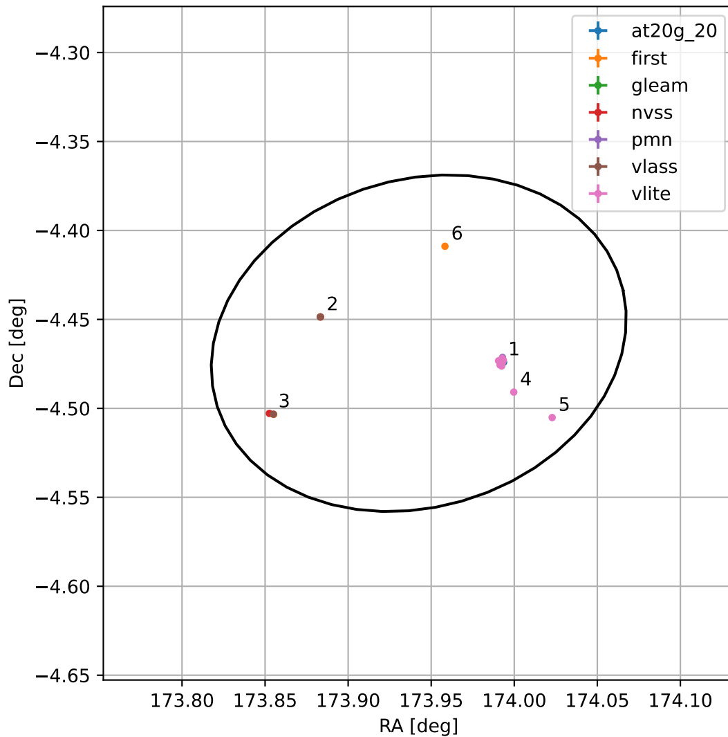
4FGL J1135.7-0427
