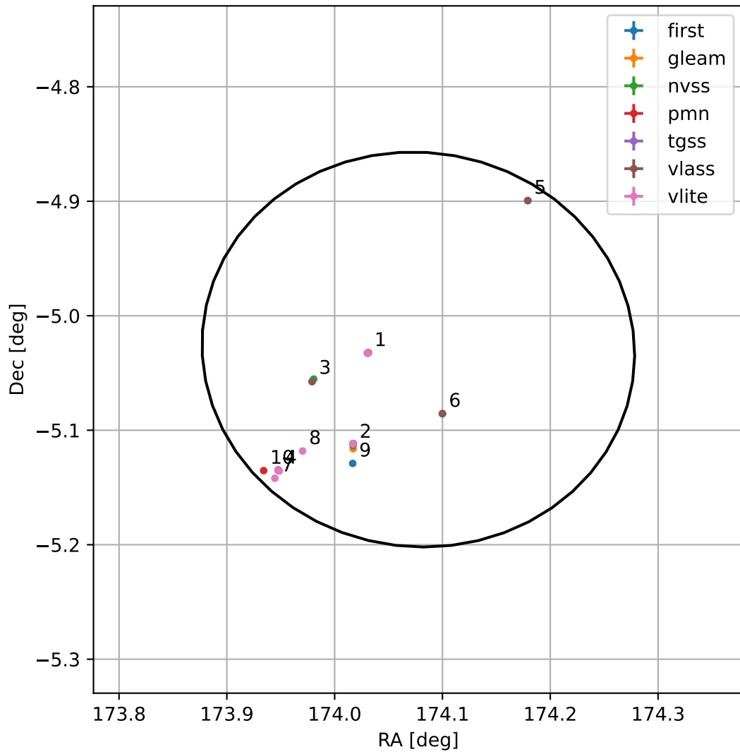
4FGL J1136.3-0501
