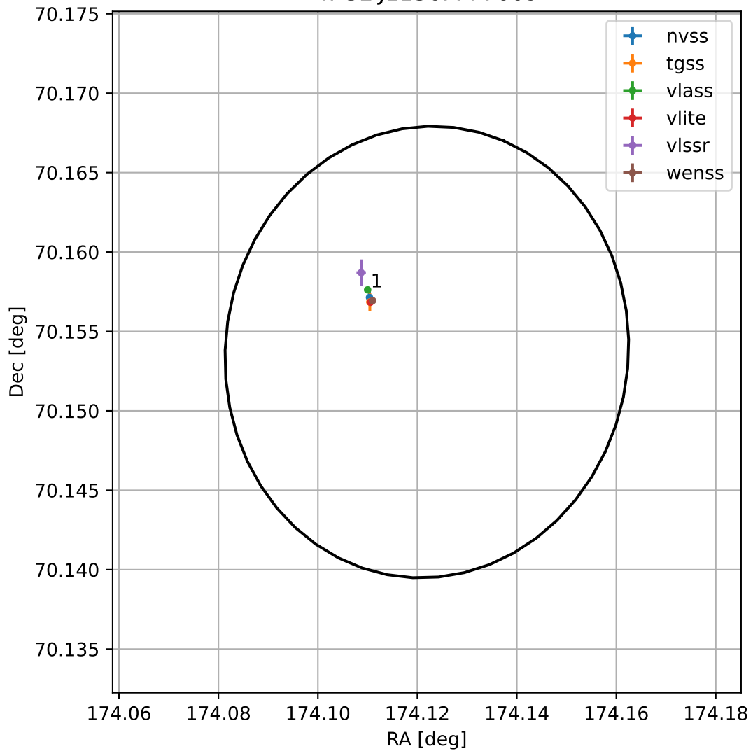
4FGL J1136.4+7009
