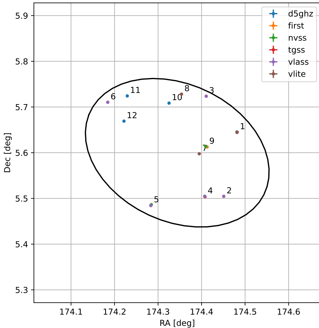
4FGL J1137.3+0535
