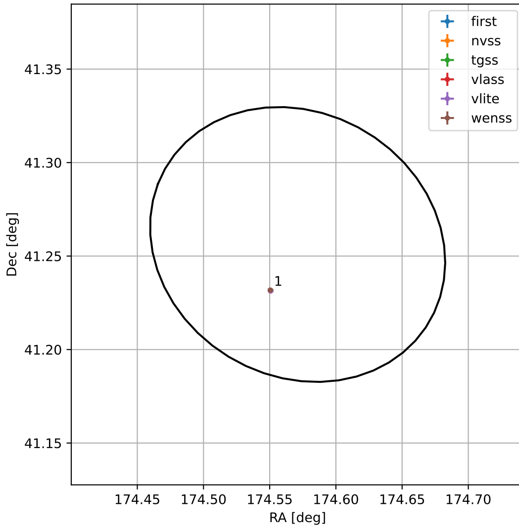
4FGL J1138.2+4115
