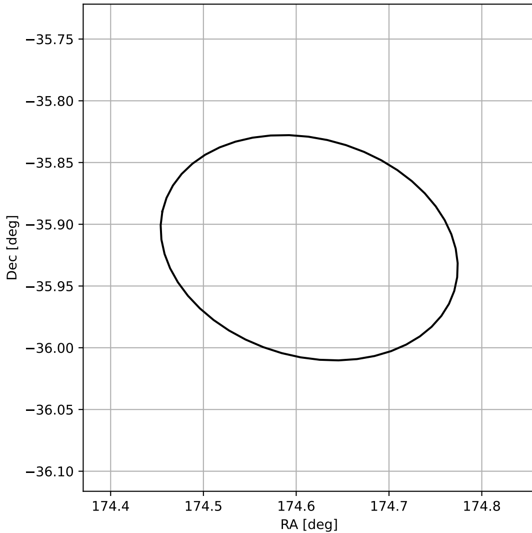
4FGL J1138.4-3555
