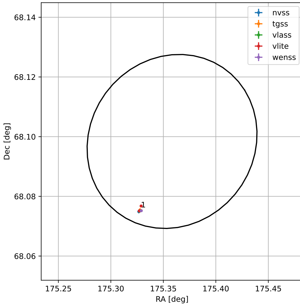
4FGL J1141.4+6805
