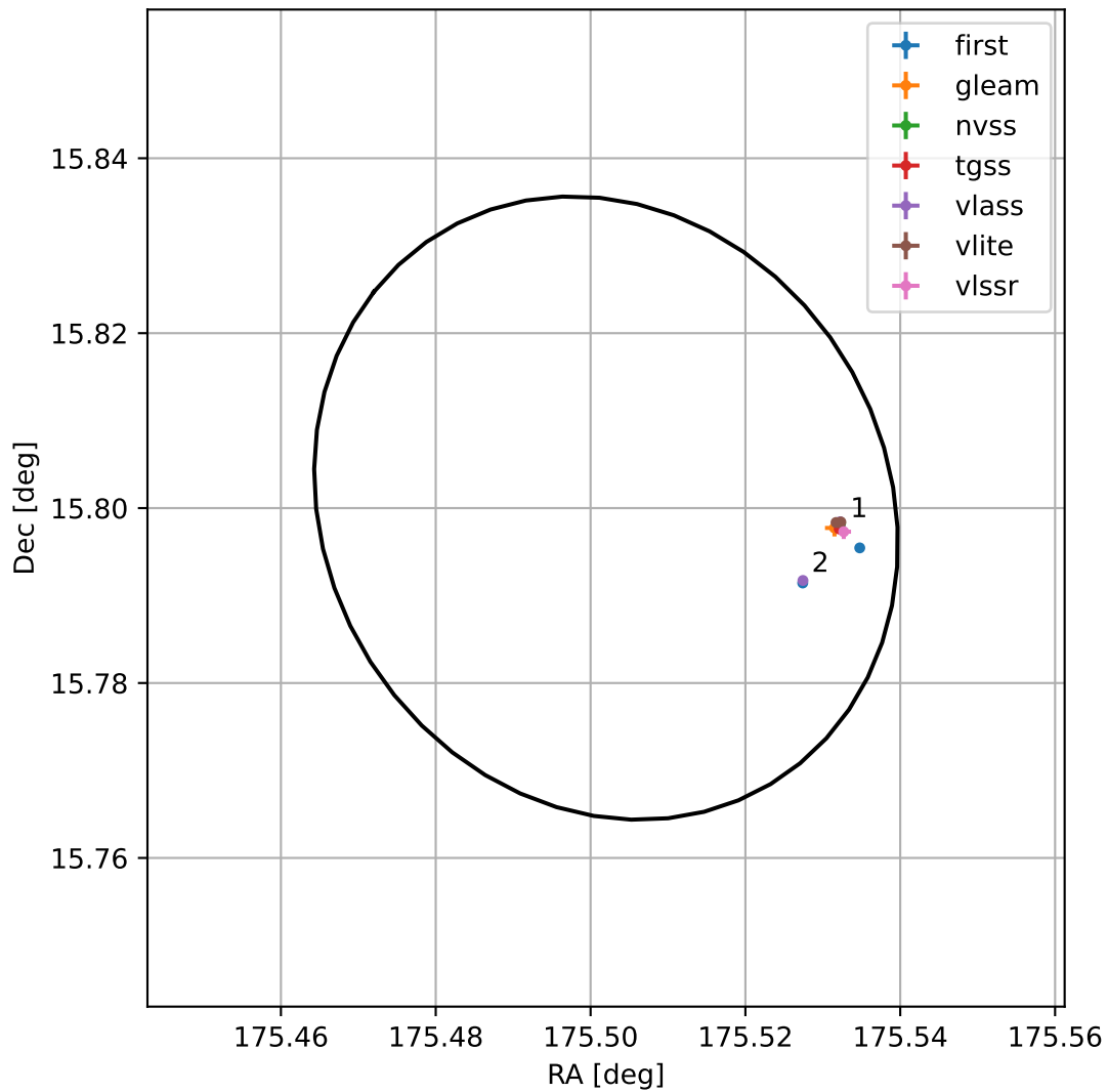
4FGL J1142.0+1548
