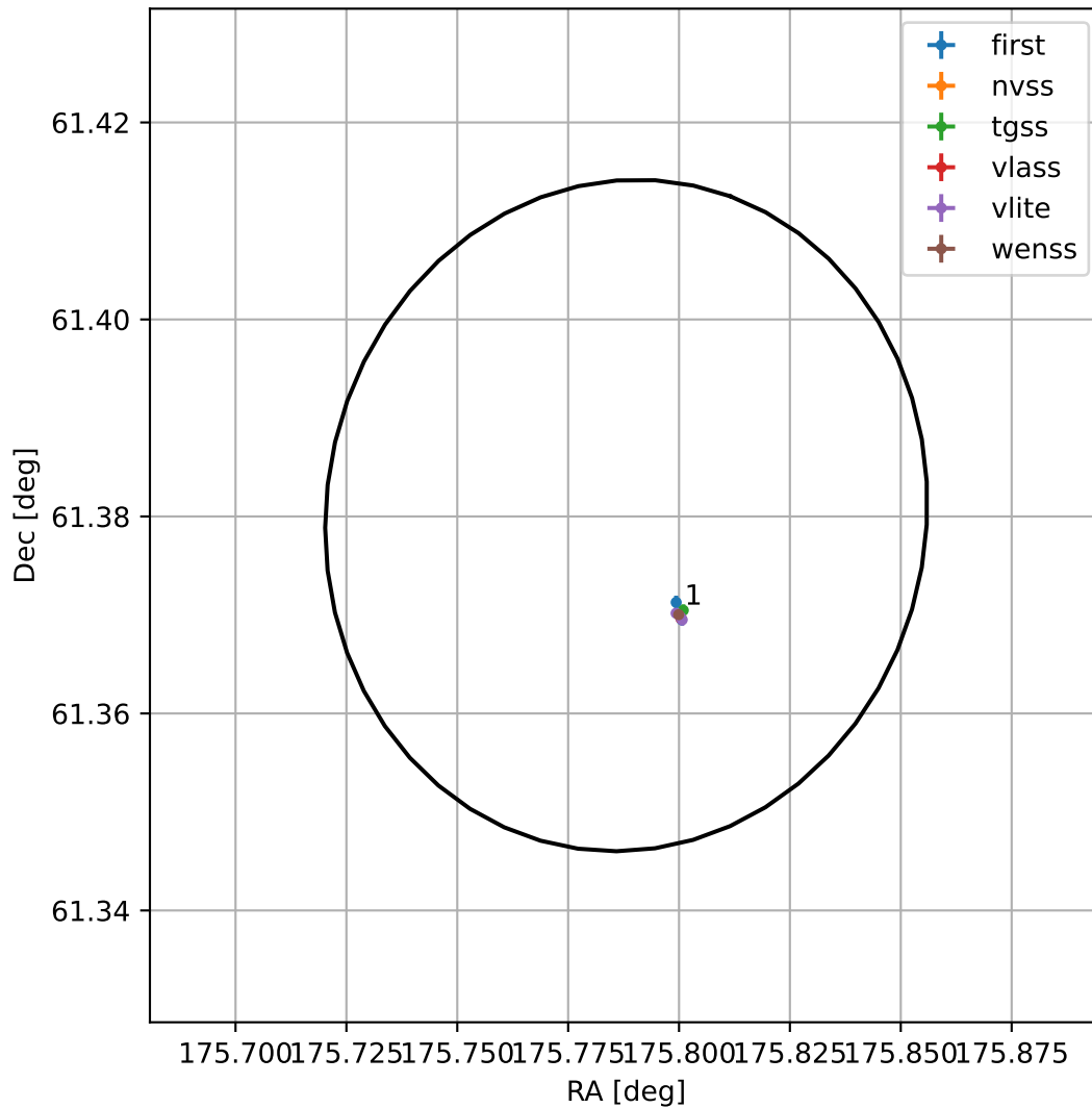
4FGL J1143.1+6122
