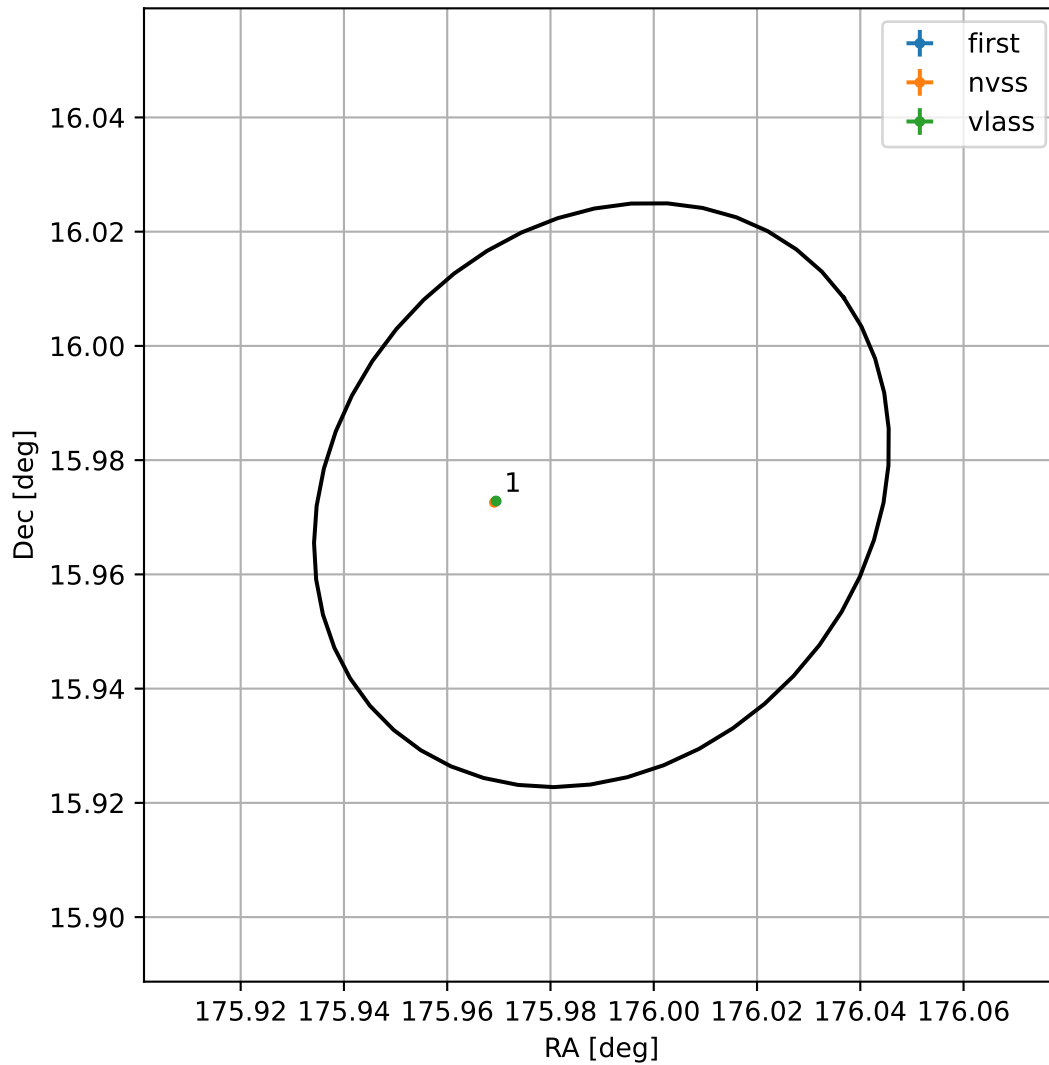
4FGL J1143.9+1558
