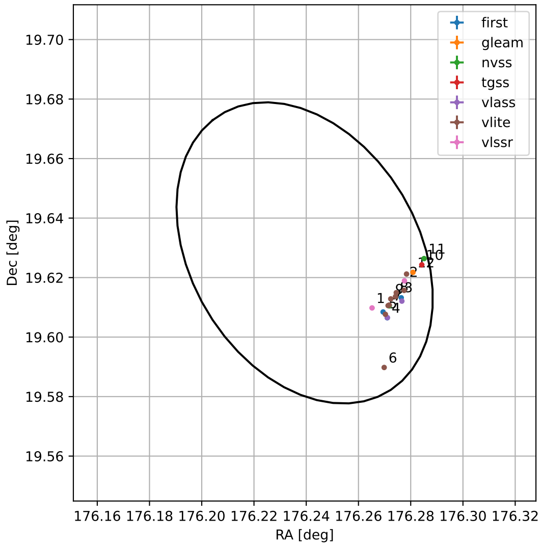
4FGL J1144.9+1937
