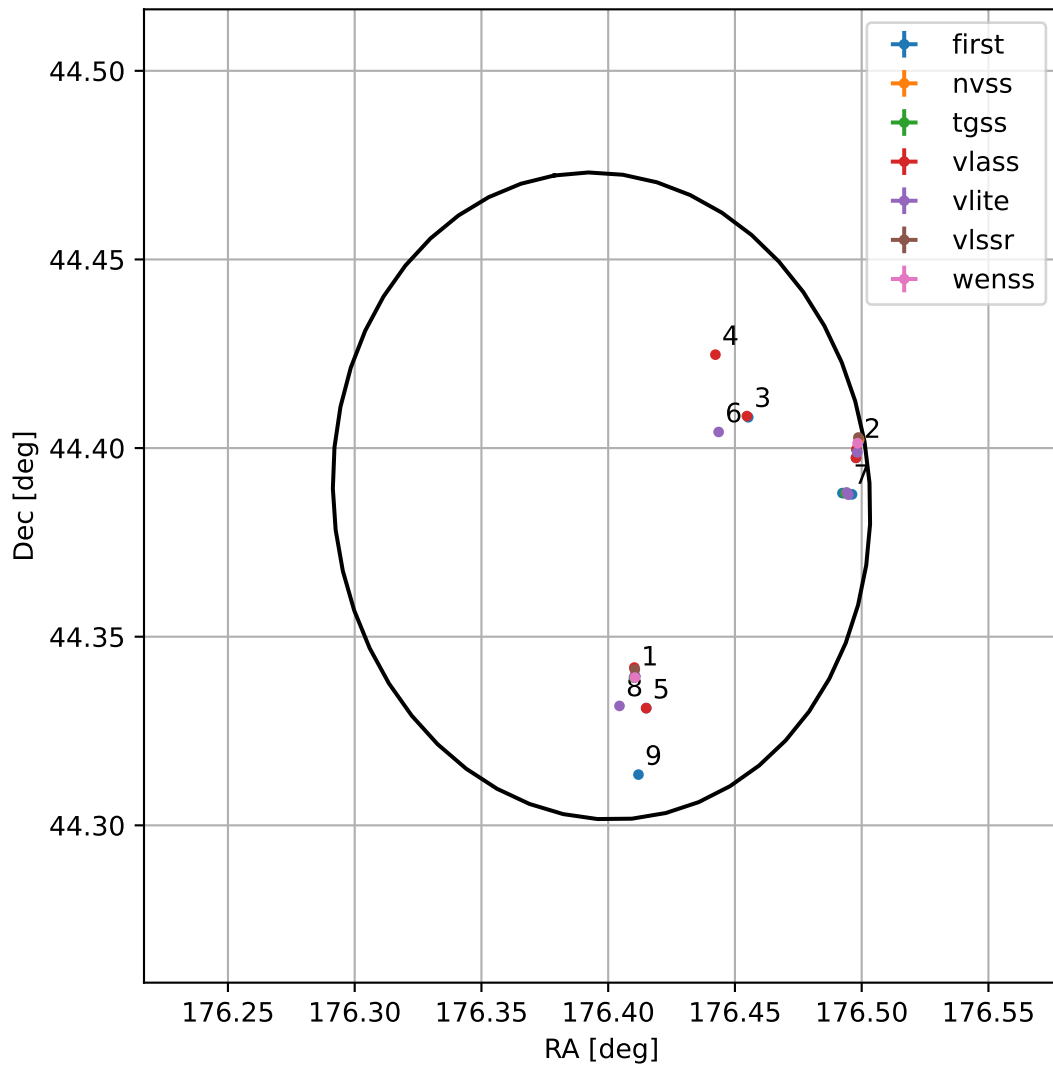
4FGL J1145.5+4423
