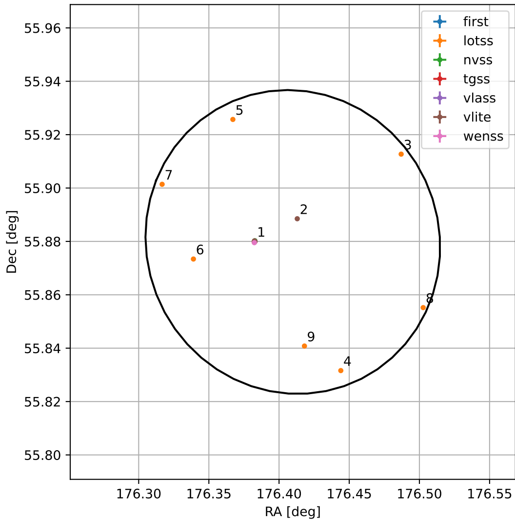
4FGL J1145.6+5552
