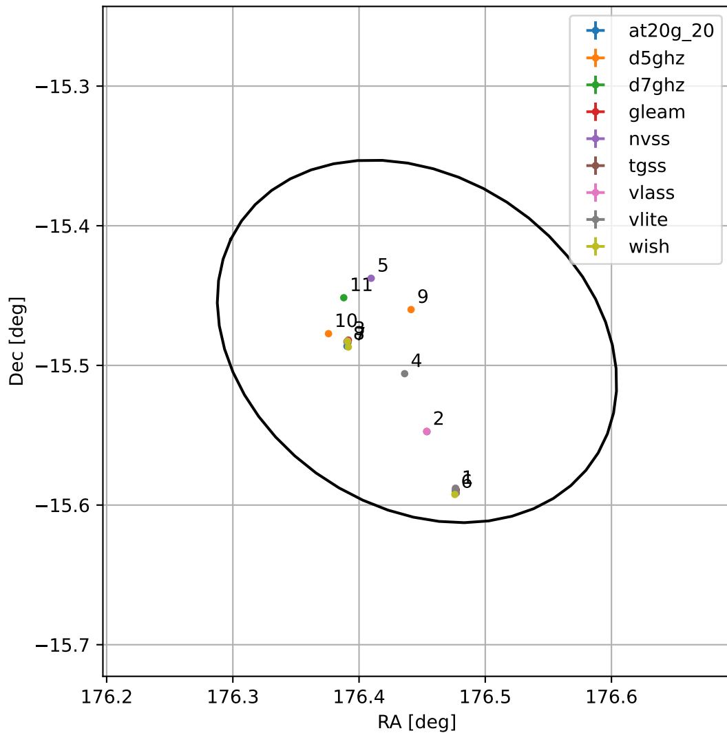
4FGL J1145.7-1528
