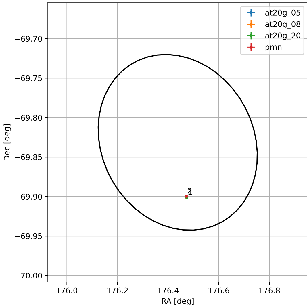
4FGL J1145.7-6949
