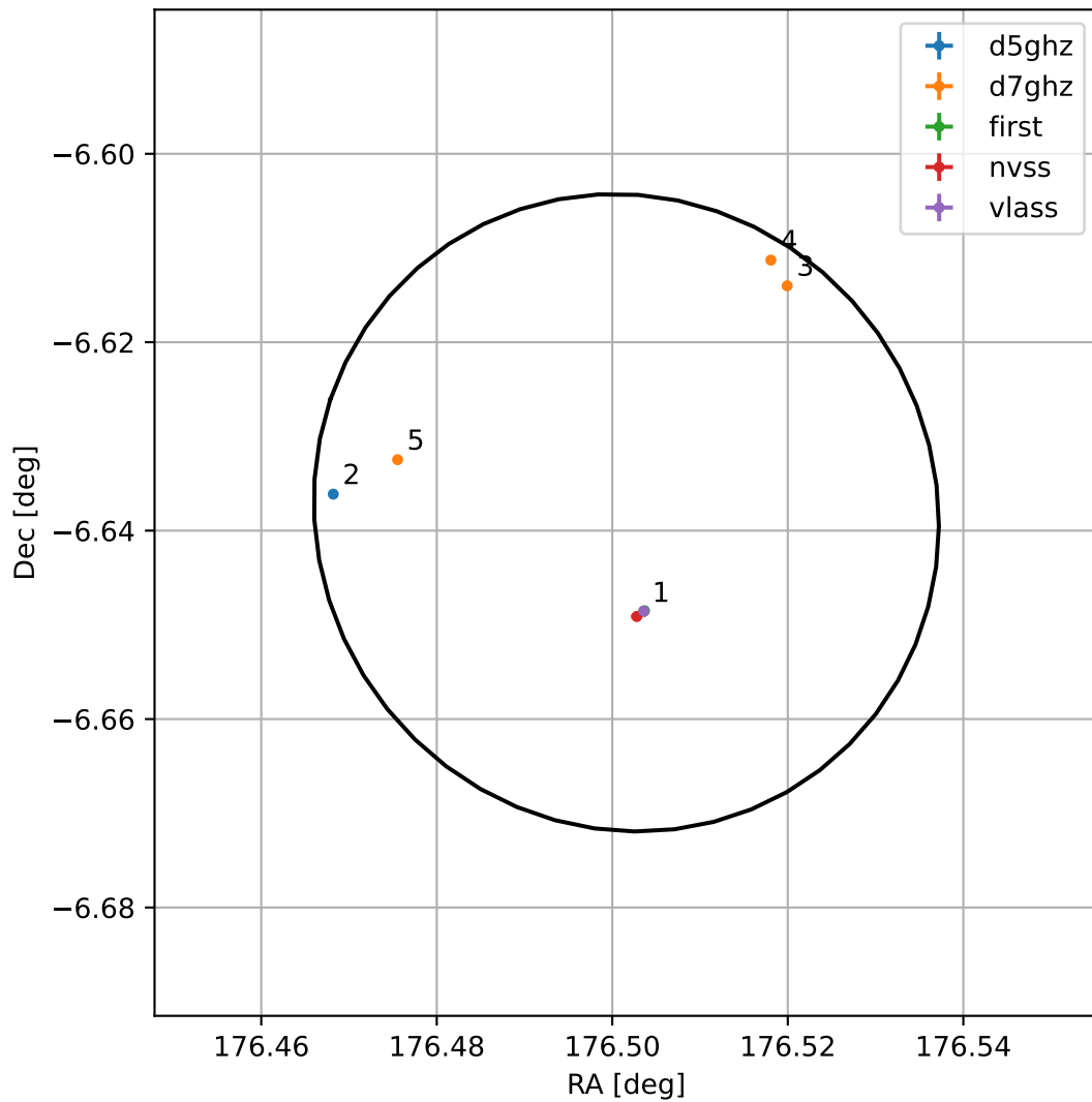
4FGL J1146.0-0638
