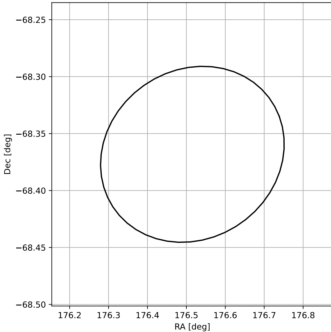
4FGL J1146.0-6822
