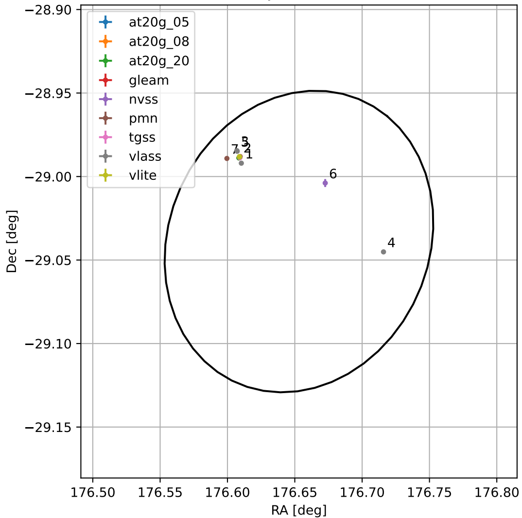
4FGL J1146.6-2902
